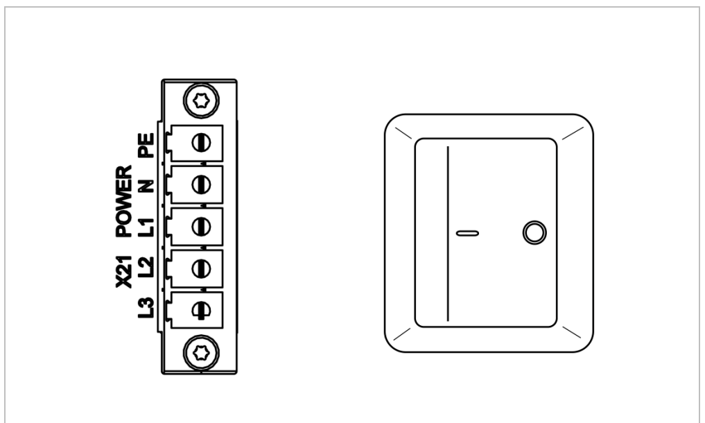
Abb. 6.5.17: X21 - Power
