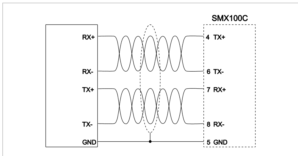
Abb. 6.5.1: COM1 – RS422
