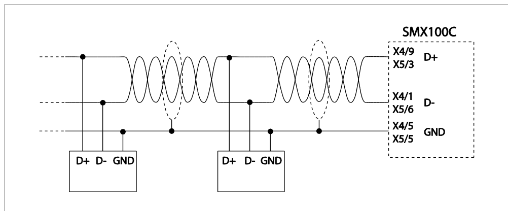
Abb. 6.5.1: COM1/COM2 – RS422
